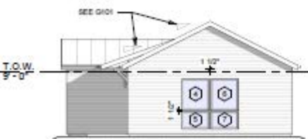
4 Side 1 Elevation 1/8" = 1'-0"
