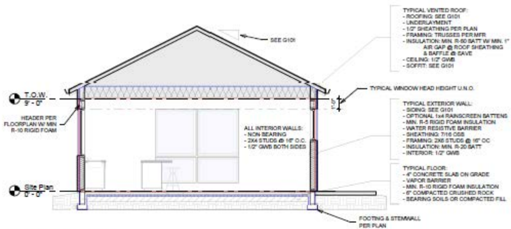
2 Typical Section 1/4" = 1'-0"
